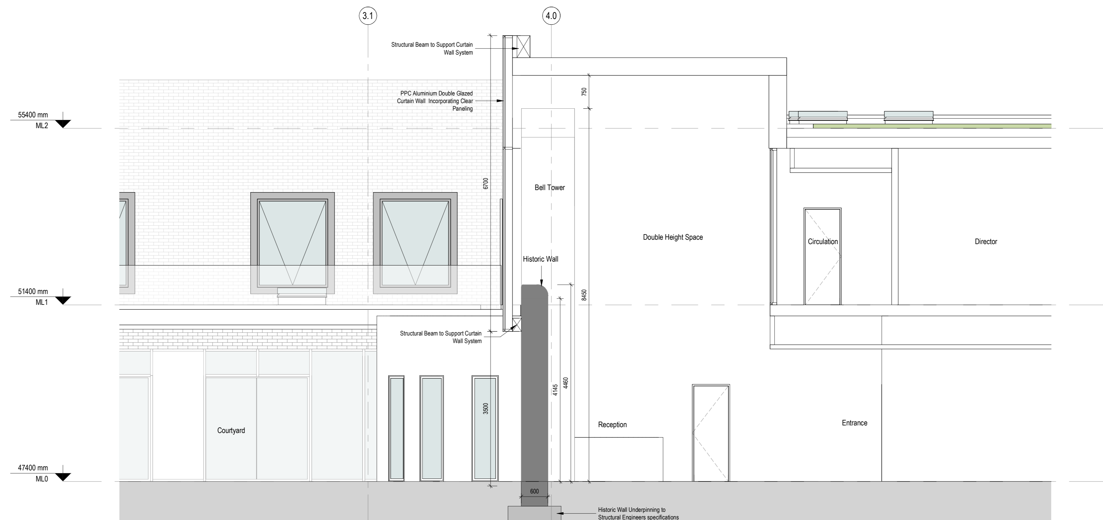
3 Section Atrium Historic Wall Scale: 1:50
